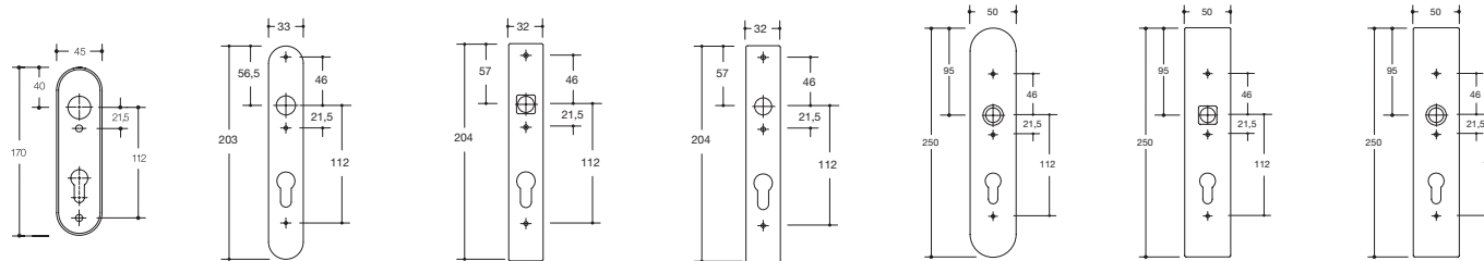
Schild 230...X..
