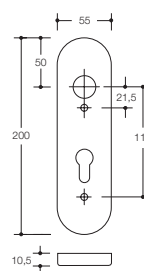
Schild 285...
